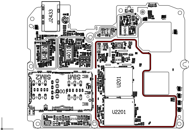
ART FILM - Assembly_Top
