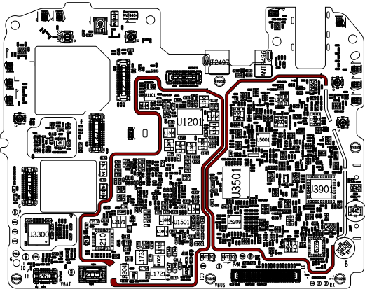
ART FILM - Assembly_Bottom
